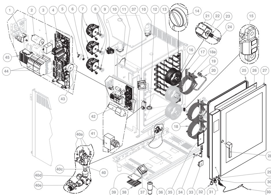
Exploded view 1/2
